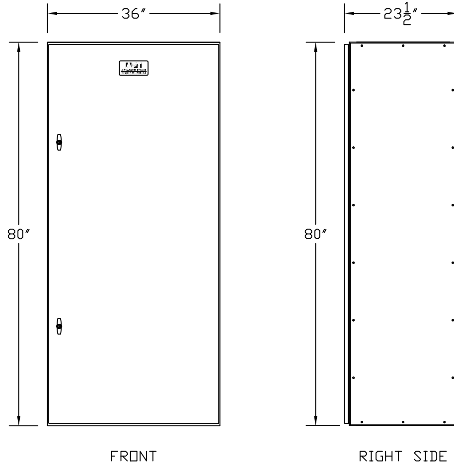
EXTERNAL VIEW (1D) - NEMA 1 WITH FRONT DOOR
