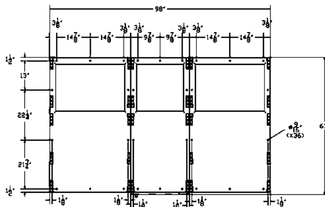
SECTION A-A (ANCHORING)
