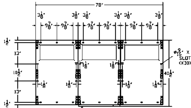
PLAN VIEW (ANCHORING)
