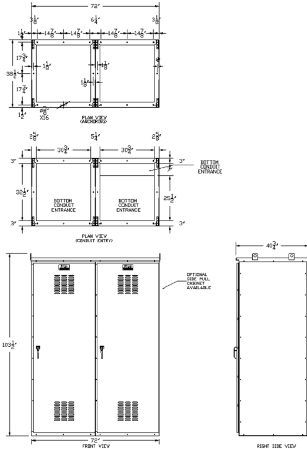
Figure 6: Two Motor Disconnects Outdoor NEMA 3R with Line & Load Side Bottom Conduit Entrance without Optional Pull Section
