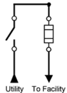
Figure 11: Utility Disconnection with Fused Overcurrent Protection
