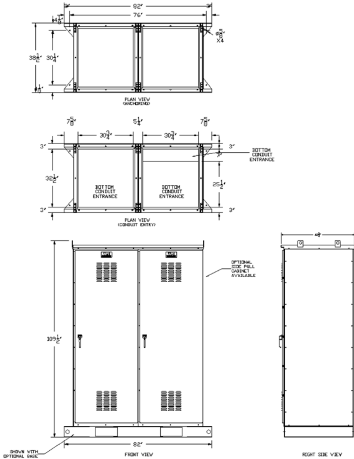
Figure 5: Two Motor Disconnects Outdoor NEMA 3R with Line & Load Side Bottom Conduit Entrance without Optional Pull Section Mounted to Switchgear Base
