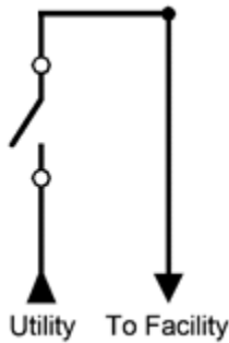
Figure 10: Utility Source Disconnection, Overcurrent Protection by Others
