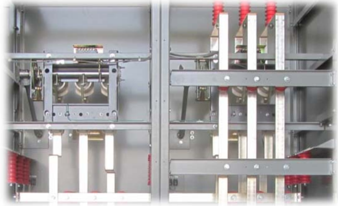
Figure 2: Optional Main bus is silver plated copper with bolted
