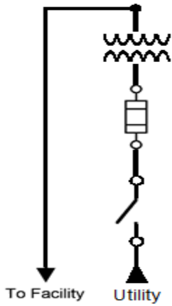
Figure 7: Transformer Primary Overcurrent Protection & Disconnection Switch
