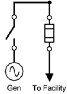
Figure 13: Generator Disconnection with Fused Overcurrent Protection
